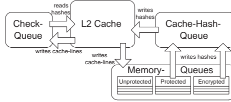
Fig. 1. Queue dependencies
